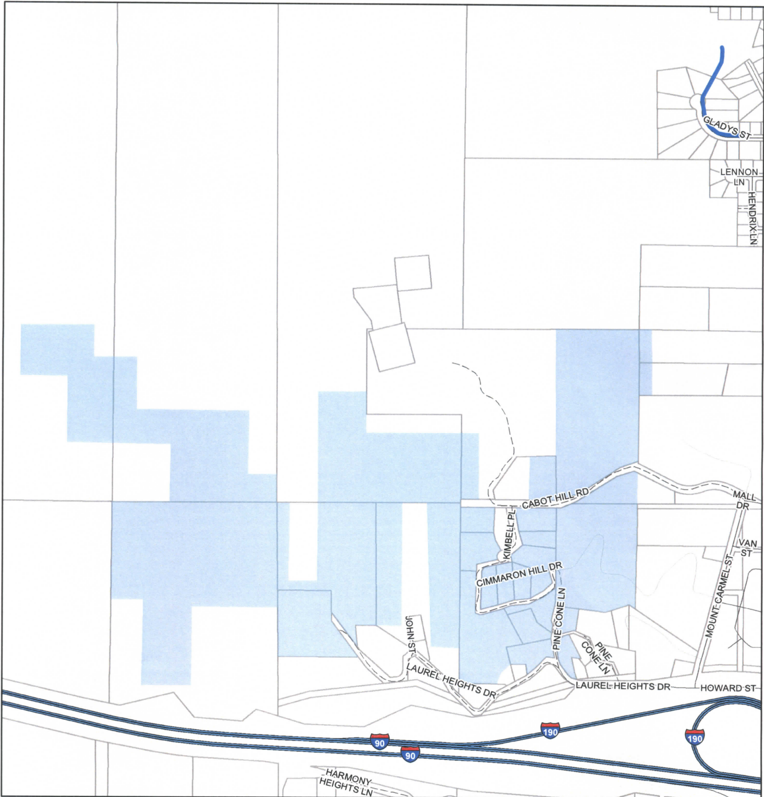
Alma St., Gladys St., and Lennon Ln. Area High Pressure South Water Main Extension Oversize City Project No. 12-2039
